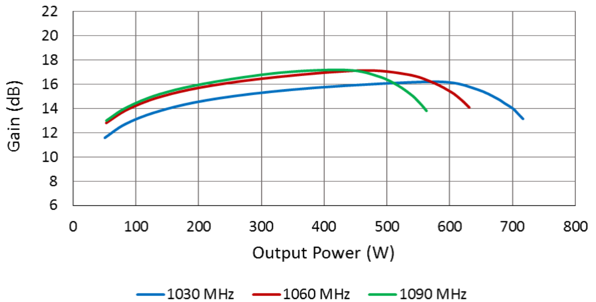
Figure 1. Power gain vs output power
