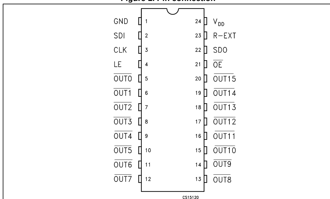
Figure 1. Pin connection
