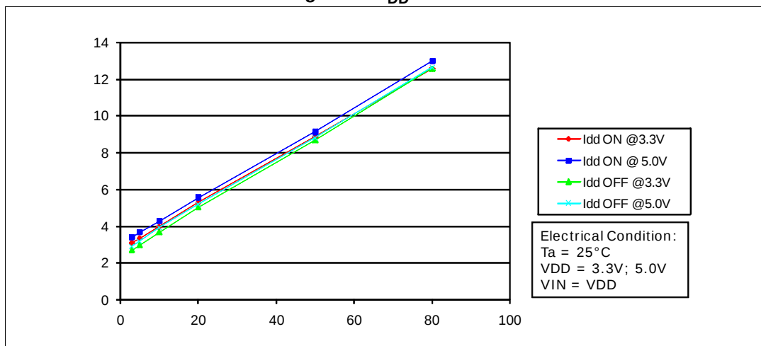
Figure 14. I_{DD} ON/OFF
