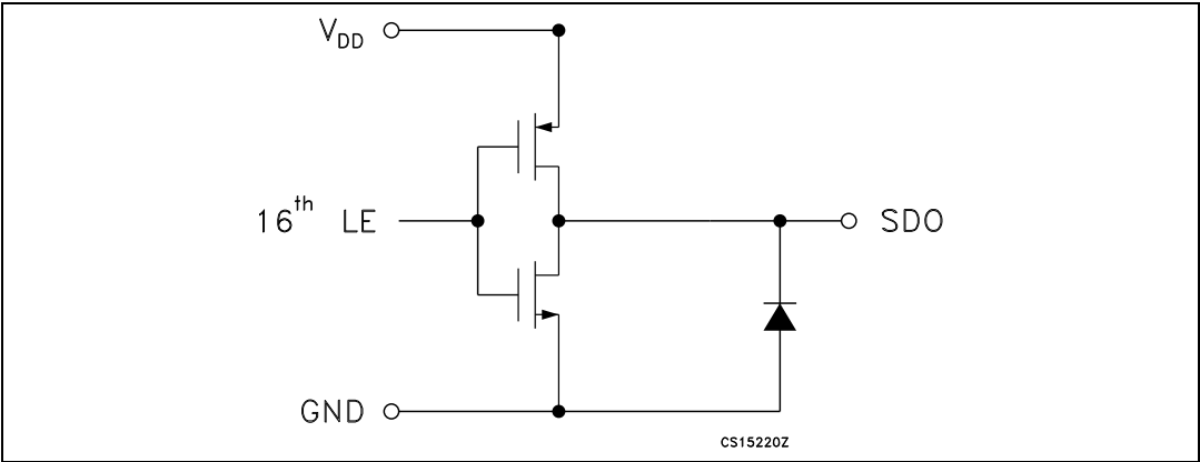
Figure 5. SDO terminal
