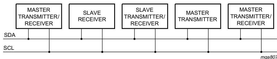
Fig 15. System configuration
