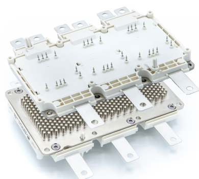
ACEPACK DRIVE
