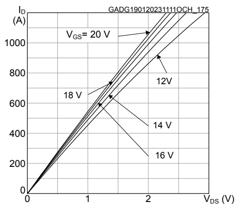
Figure 3. Typical output characteristics ( T_J = 175\text{ }^{\circ}\text{C} )
