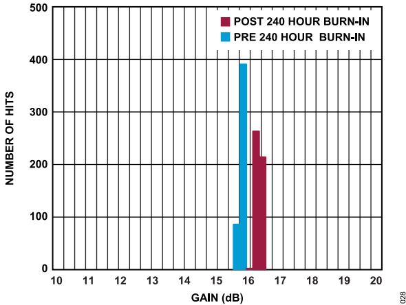
Figure 28. Gain Distribution Before and After 240 Hour Burn-in, Frequency = 1 GHz
