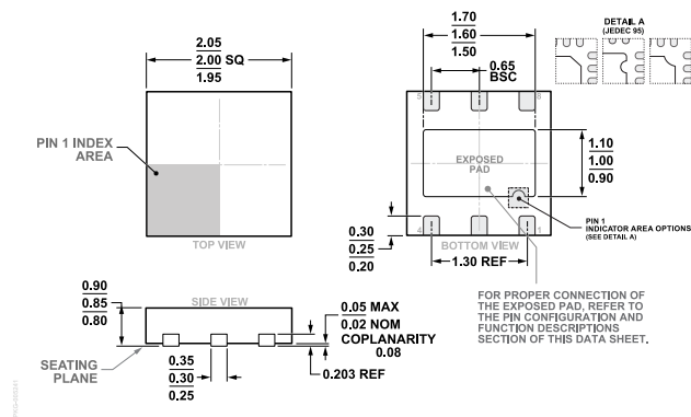
Figure 29. 6-Lead Lead Frame Chip Scale Package [LFCSP] 2 mm x 2 mm Body and 0.85 mm Package Height (CP-6-12) Dimensions shown in millimeters
