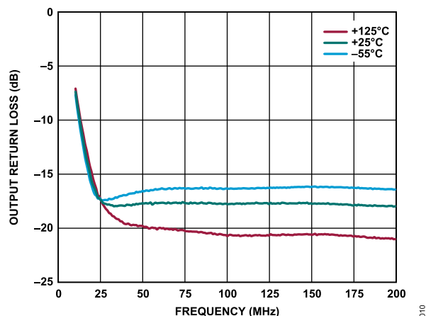
Figure 10. Output Return Loss vs. Frequency, 10 MHz to 200 MHz, for Various Temperatures, V_{DD} = 5\text{ V} , I_{DQ} = 55\text{ mA}
