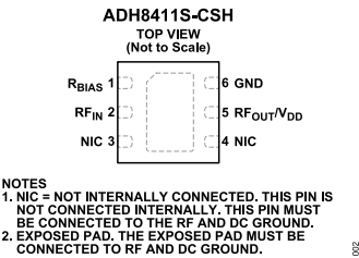
Figure 3. Pin Configuration
