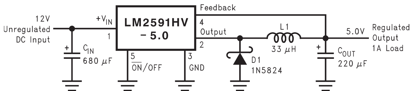
Figure 28. Typical Application
