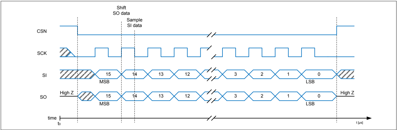
Figure 13 Communication frame
