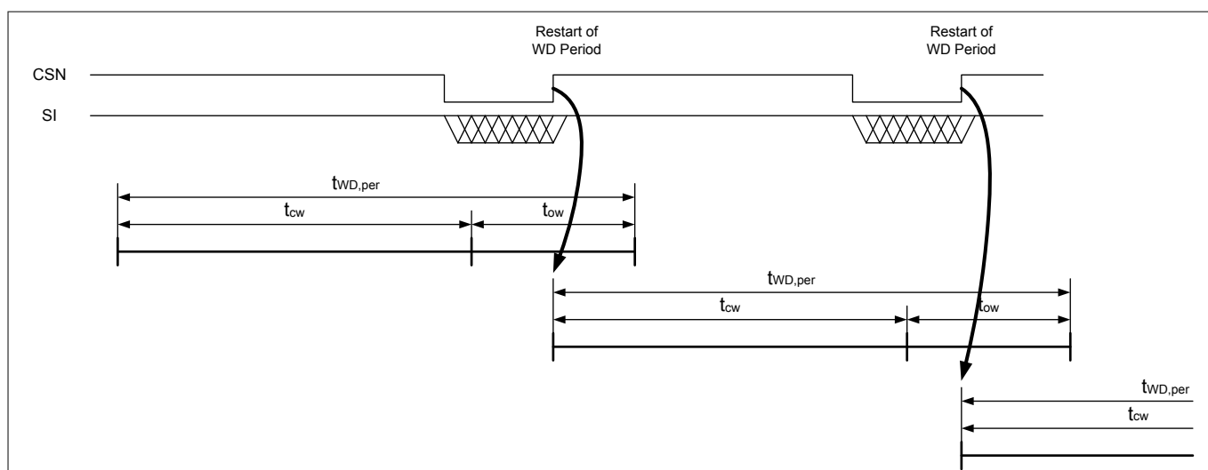
Figure 7 Watchdog trigger
