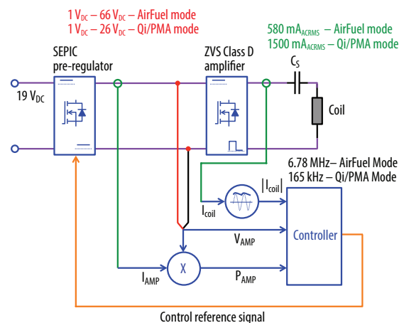
Figure 2: Block diagram of EPC9511 multi-mode capable wireless power amplifier controller.
