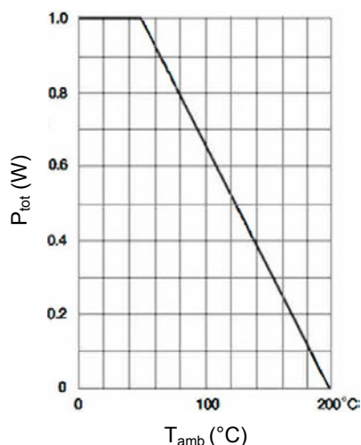
Figure 1. Admissible Power Dissipation vs. Ambient Temperature
