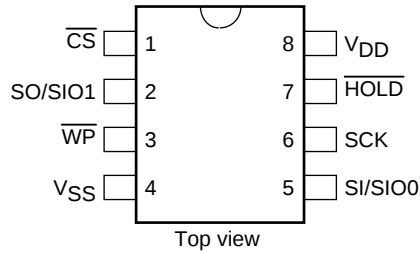
Figure 1. Pin Assignments
