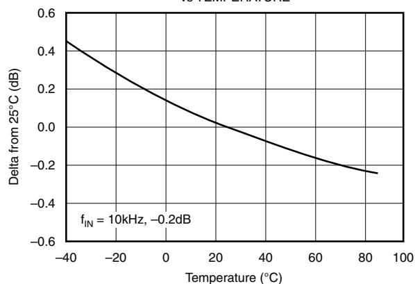
CHANGE IN SIGNAL-TO-(NOISE+DISTORTION) vs TEMPERATURE
