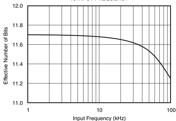
EFFECTIVE NUMBER OF BITS vs INPUT FREQUENCY
