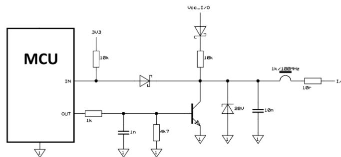
Figure 2. I/O Circuitry
