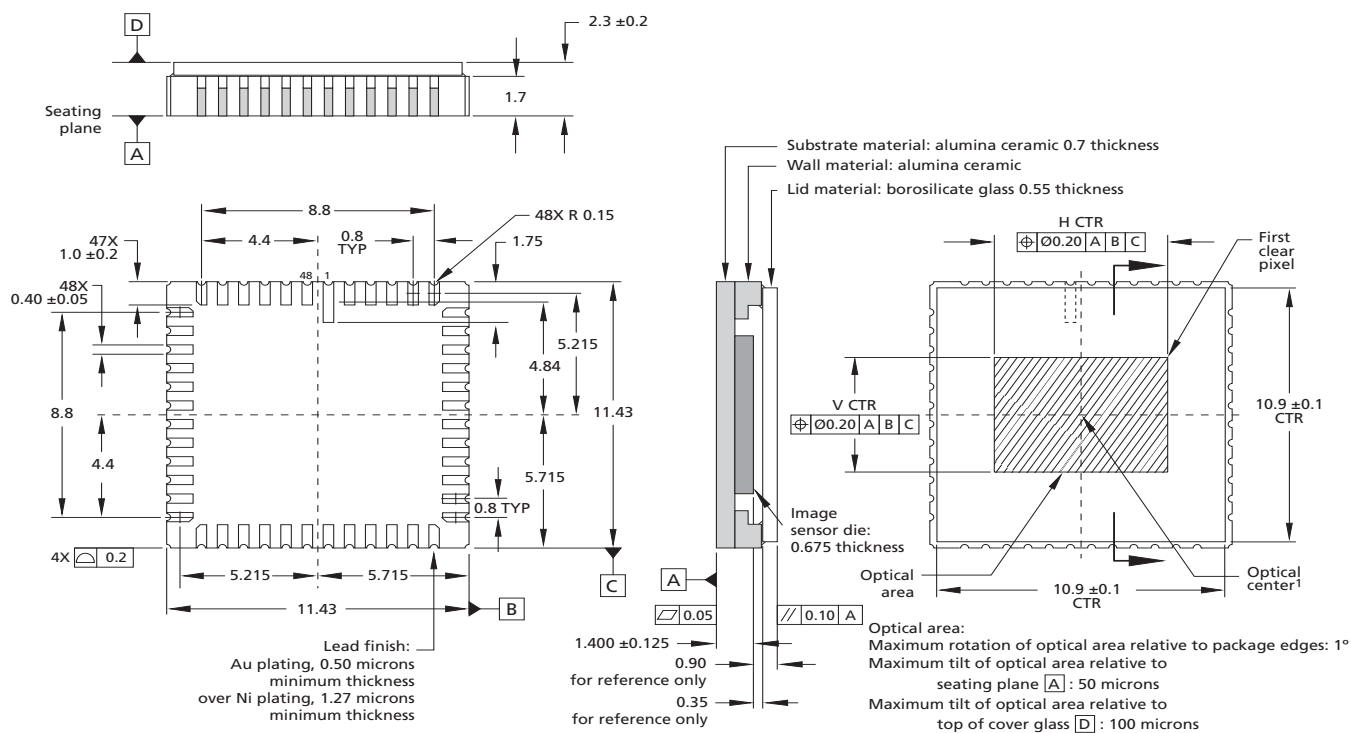
Figure 10: 48-Pin CLCC Package Outline Drawing
