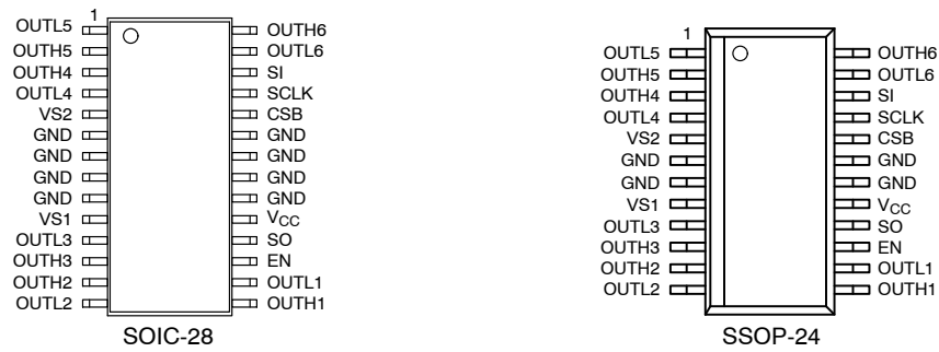
Figure 2. Pin Connection
