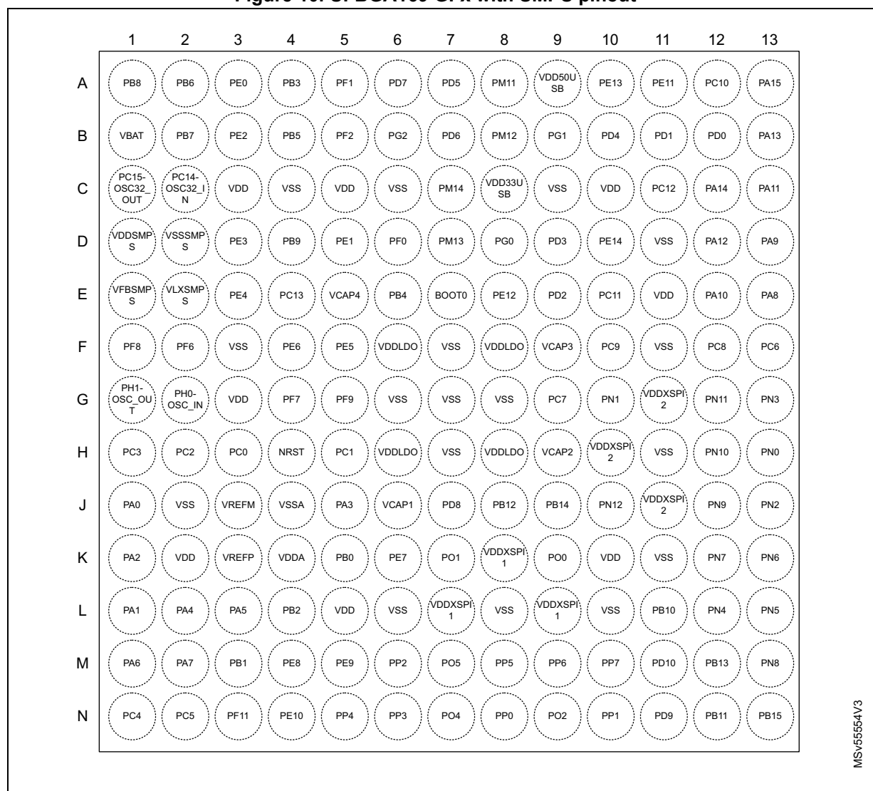
Figure 10. UFBGA169 GFx with SMPS pinout (a)
