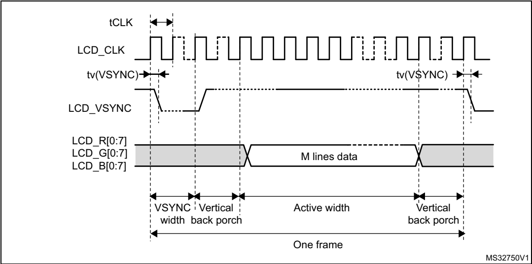
Figure 60. LCD-TFT vertical timing diagram
