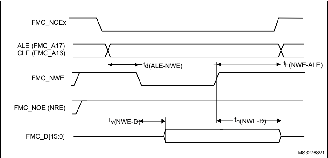
Figure 48. NAND controller waveforms for write access
