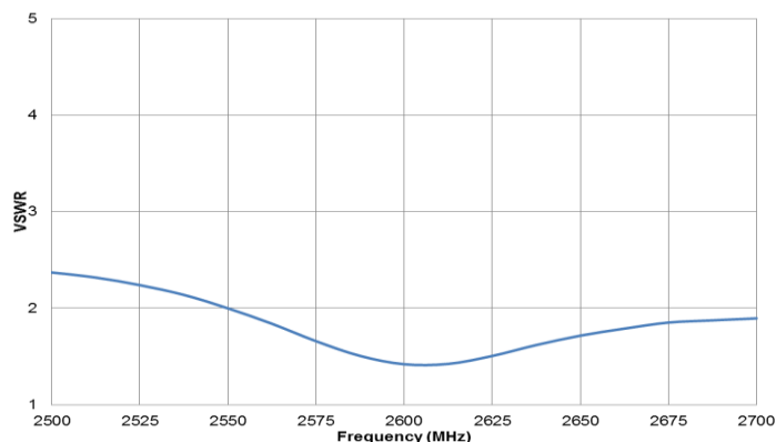
Band 7 VSWR
