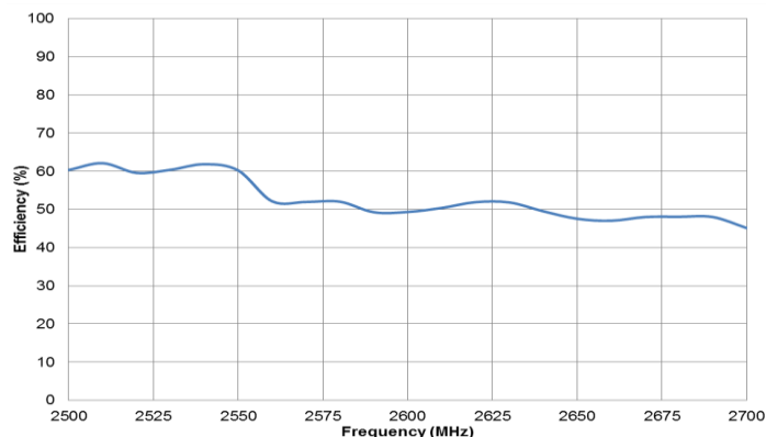
Band 7 Efficiency
