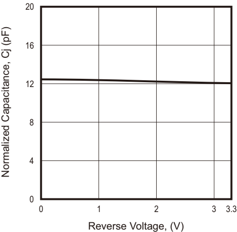
Fig.6 - Junction Capacitance Vs. Reverse Voltage
