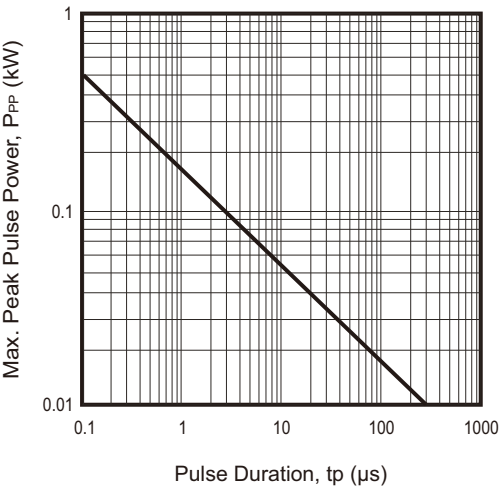
Fig.2 - Non-Repetitive Max. Peak Pulse Power vs. Pulse Time
