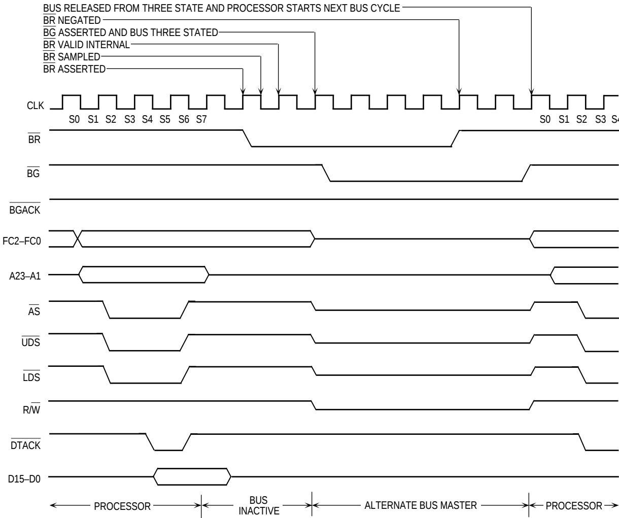
Figure 5-23. 2-Wire Bus Arbitration Timing Diagram—Bus Inactive
