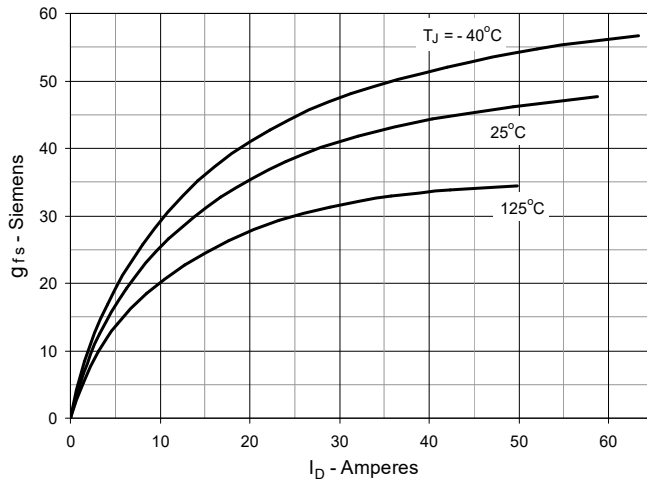
Fig. 9. Transconductance
