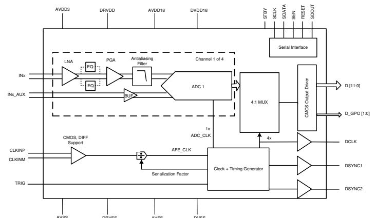
Simplified Schematic
