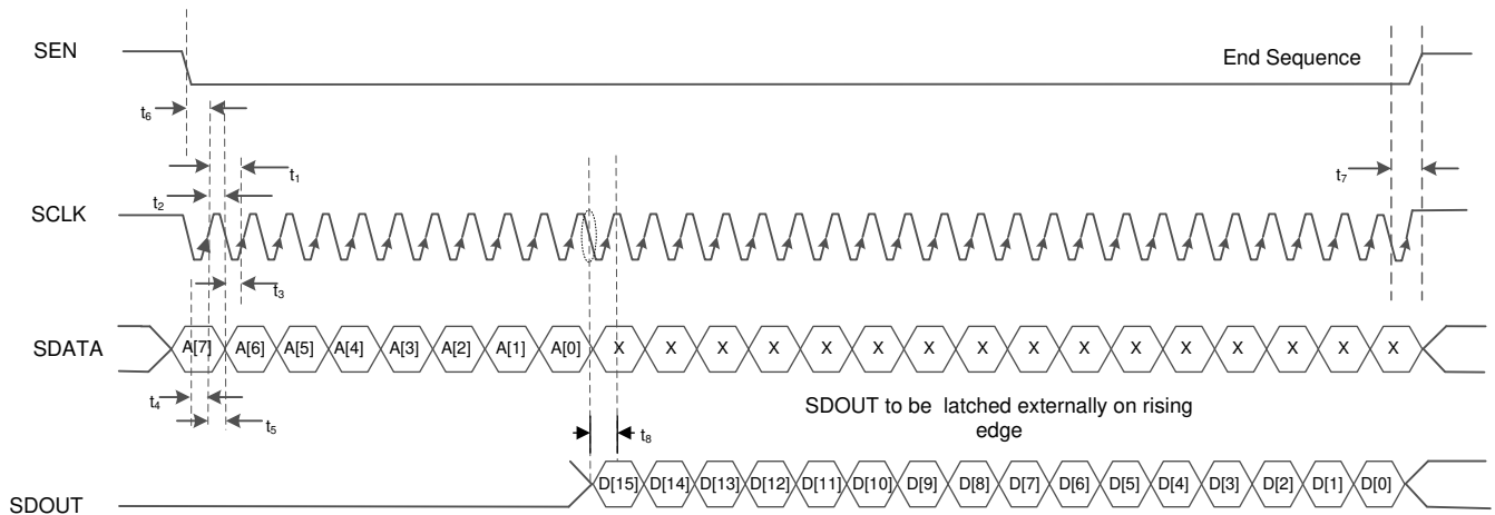
Figure 5-4. Serial Interface Register Readout Timing Diagram
