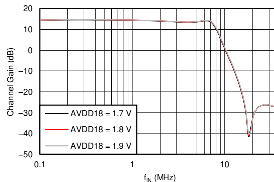
Figure 5-34. Antialias Filter Response vs AVDD18 (PGA Gain = 0 dB, FILTER_BW = 8 MHz)
