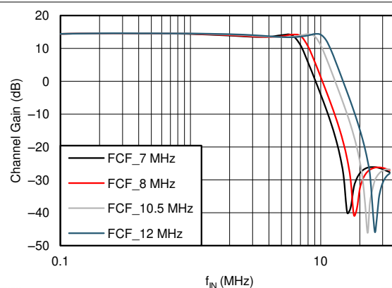
Figure 5-32. Antialias Filter Response vs FILTER_BW Settings (PGA Gain = 0 dB)
