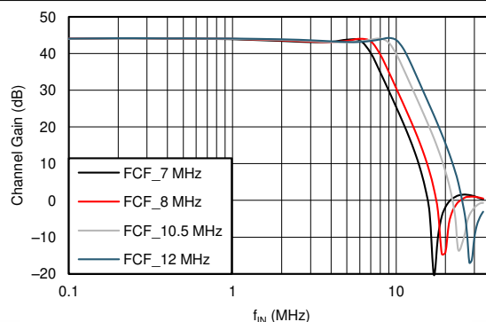
Figure 7-3. Filter Response Across Modes (PGA Gain = 30 dB)
