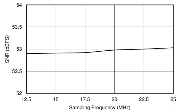
Figure 5-20. Signal-to-Noise Ratio vs Sampling Frequency (PGA Gain = 30 dB)
