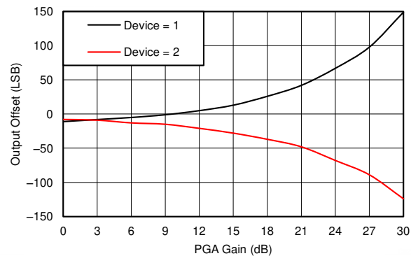
Figure 5-30. Channel Offset vs PGA Gain for Two Typical Devices
