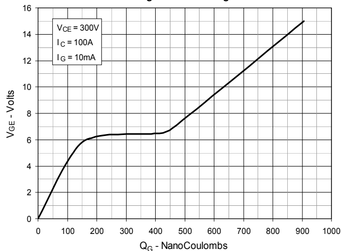
Fig. 7. Gate Charge
