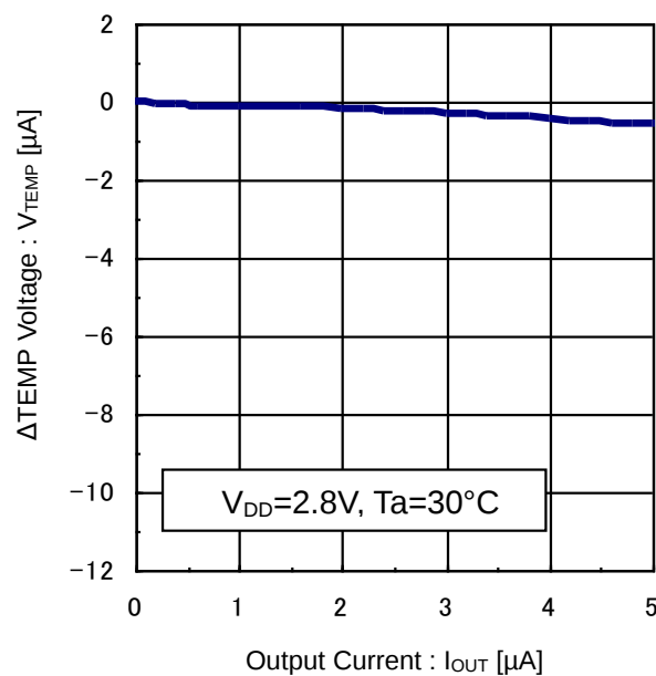
Figure 4. TEMP Voltage vs Output Current
