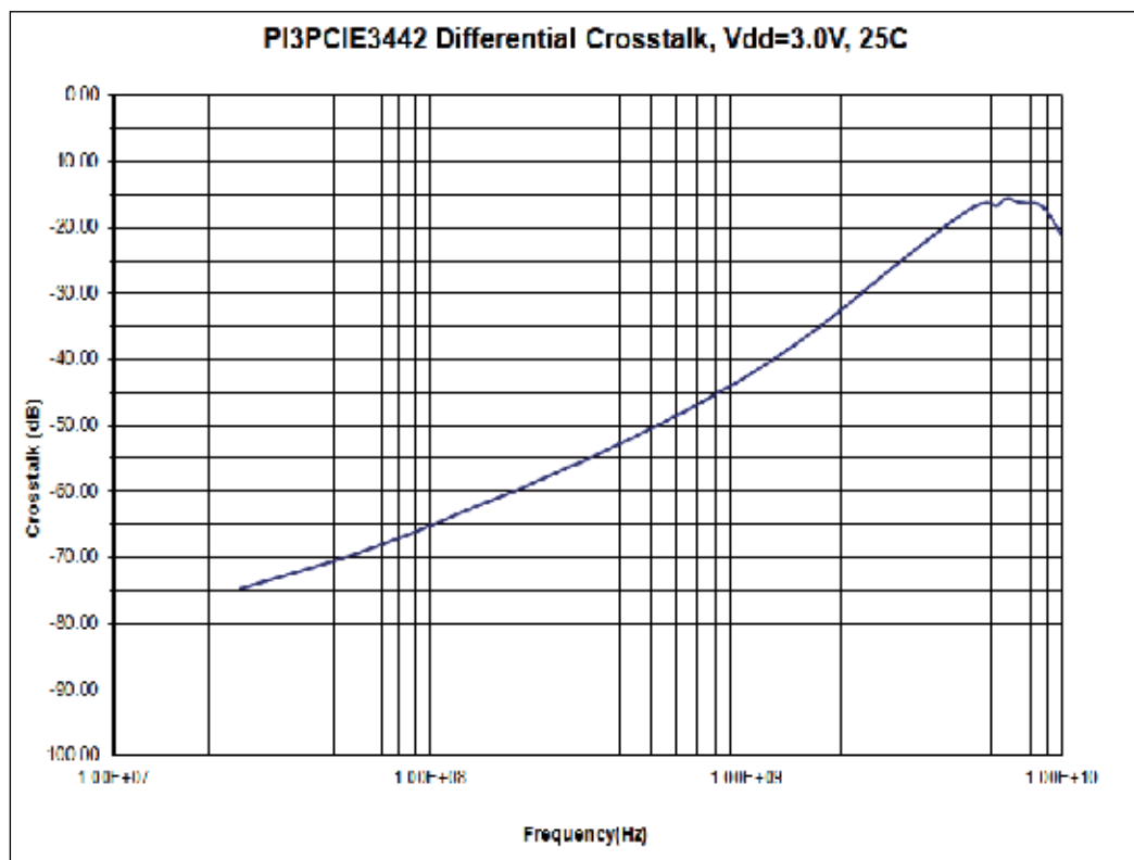
Differential Crosstalk
