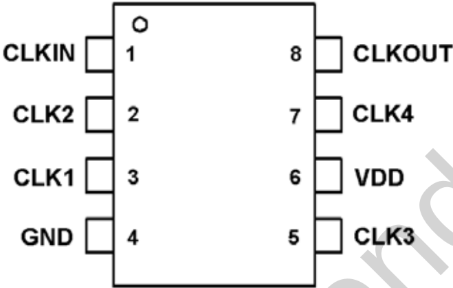
Figure 5. 8-Pin SOIC
