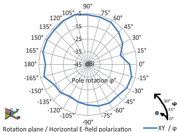
Fig. 4 - VJ5301M868MXBSR XY Radiation Pattern
