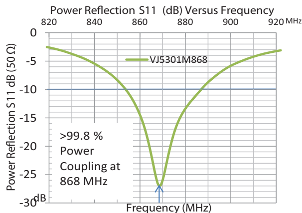
Fig. 2 - VJ5301M868 Tuned to 868 MHz with > 99.8 % Power Coupled
