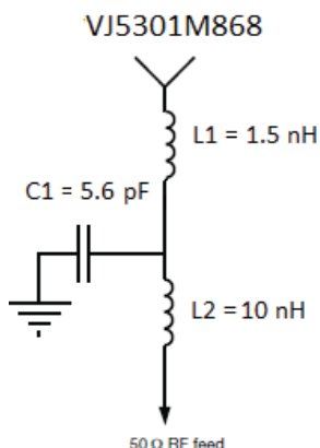
Fig. 1 - Tuning Example with Inductors L1, L2 and Capacitor C1
