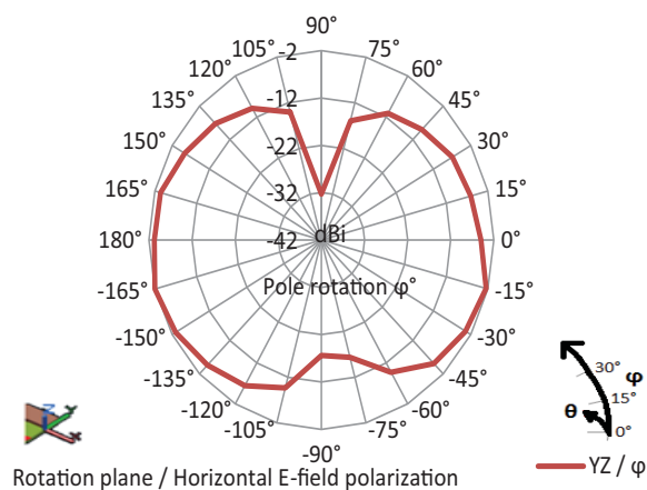
Fig. 5 - VJ5301M868MXBSR YZ Radiation Pattern
