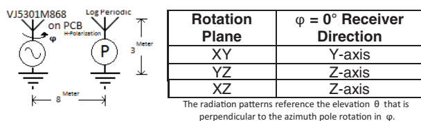
Fig. 3 - VJ5301M868 PCB Mounting and Coordinate Directions
