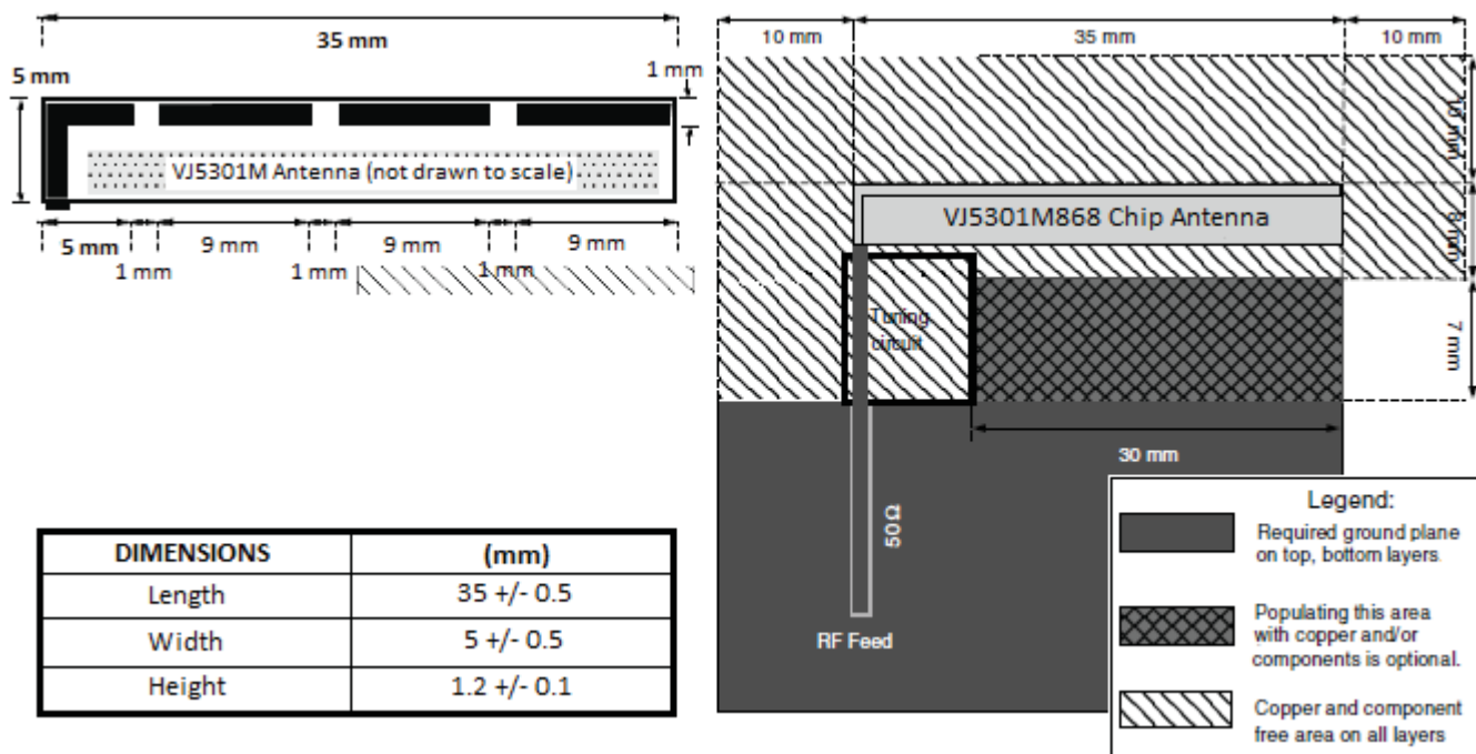
Fig. 7 - Footprint, Chip Antenna Mechanical Dimensions, and PCB Layout Dimensions of VJ5301M868
