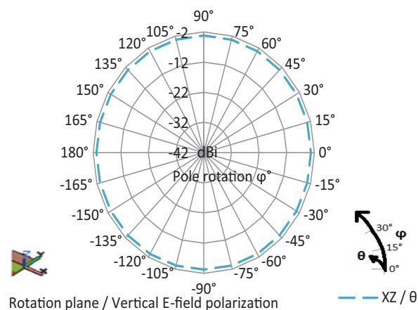
Fig. 6 - VJ5301M868MXBSR XZ Radiation Pattern
