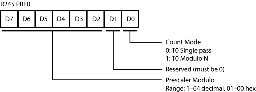
Figure 36. Prescaler 0 Register (F5H: Write Only)
