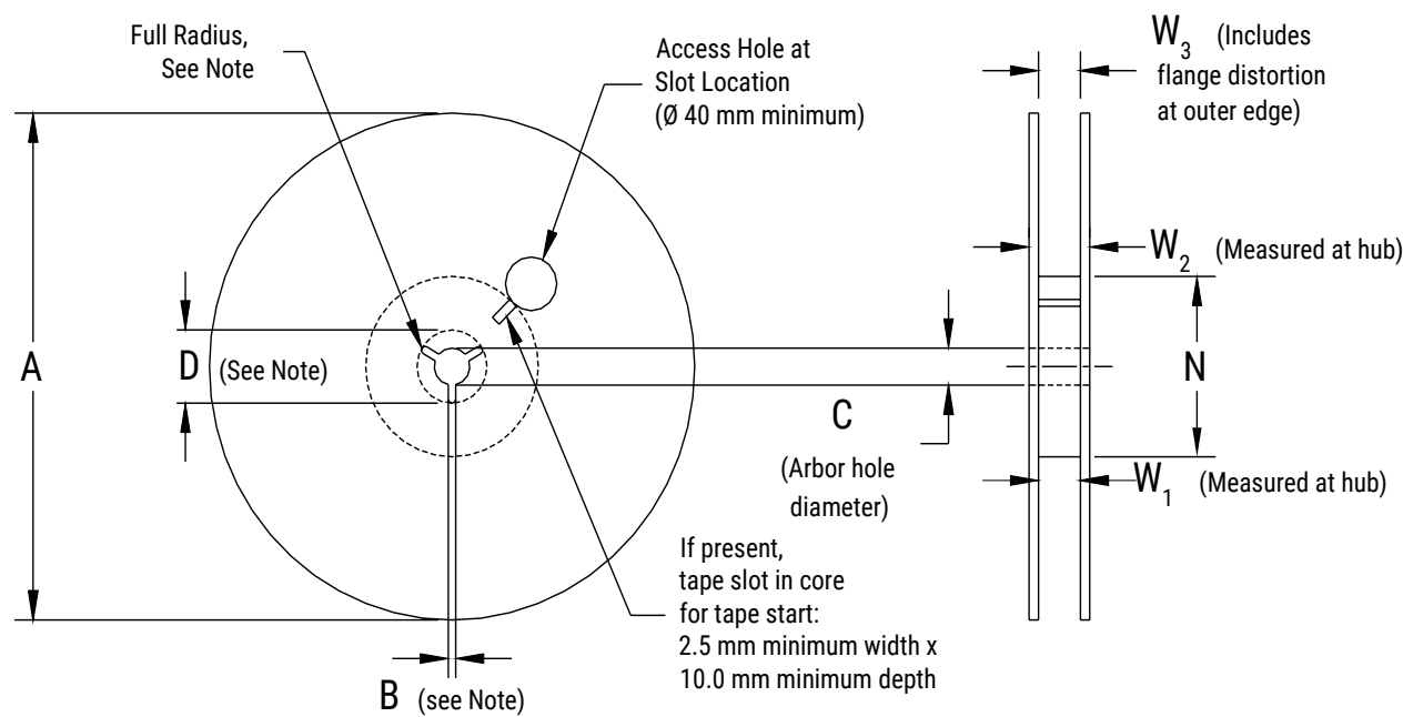
Figure 6 – Reel Dimensions
