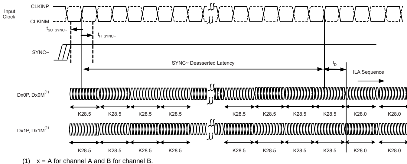
Figure 5. SYNC~ Latency in ILAS Phase (Two-Lane Mode)
