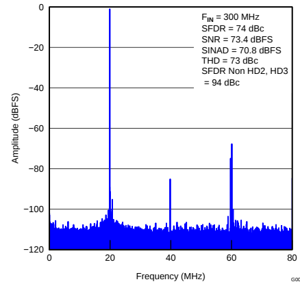
Figure 11. FFT for 300-MHz Input Signal (2.5- V_{\text{PP}} Full-Scale)
