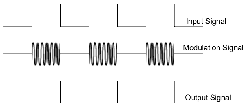
Figure 6. Modulation Scheme
