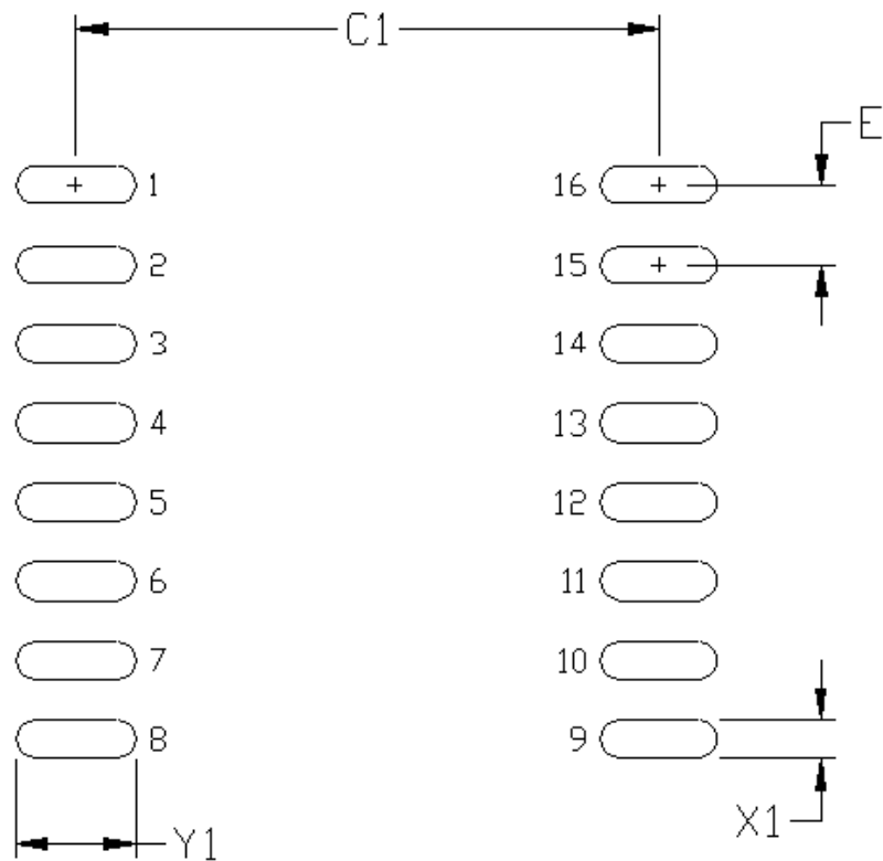
Figure 42. 16-Pin Wide-Body SOIC Land Pattern Drawing
