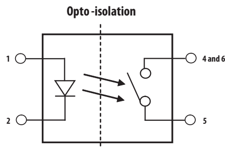
Equivalent Relay Diagram
