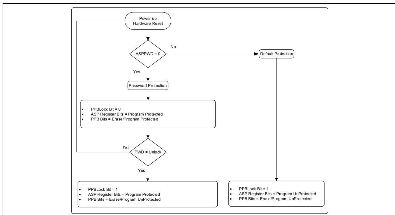
Figure 29 Password protection scheme flowchart
