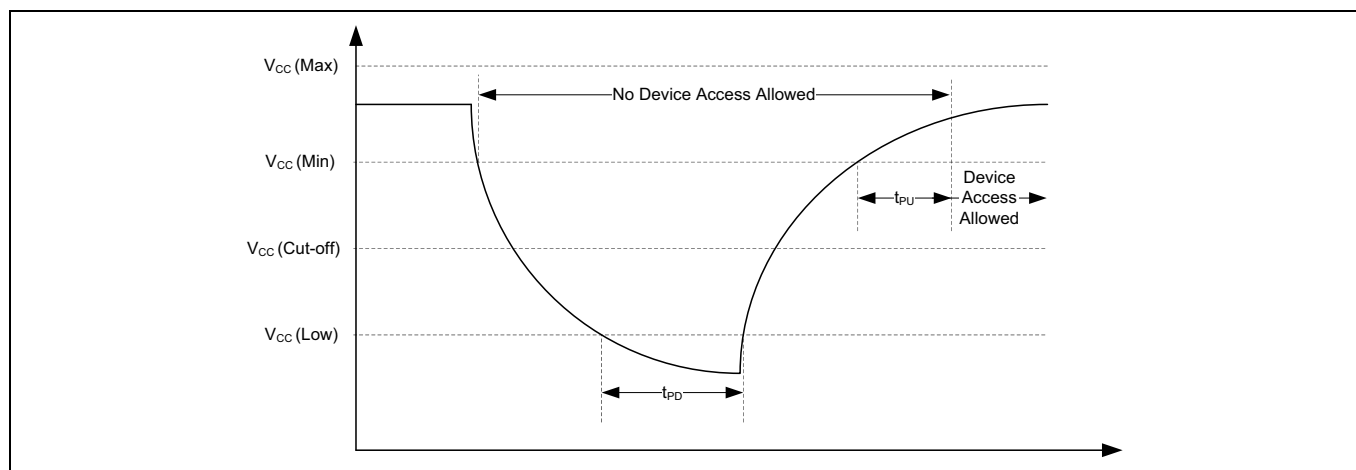
Figure 48 Power down and voltage drop
