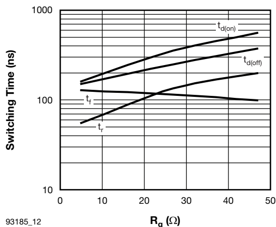
Fig. 12 - Typical IGBT Switching Time vs. R_g T_J = 125^\circ\text{C} , L = 500\text{ }\mu\text{H} , V_{CC} = 360\text{ V} , I_C = 100\text{ A} , V_{GE} = 15\text{ V}
