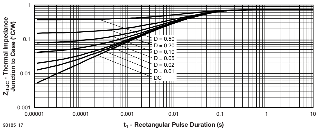
Fig. 17 - Maximum Thermal Impedance Z_{thJC} Characteristics (Diode)
