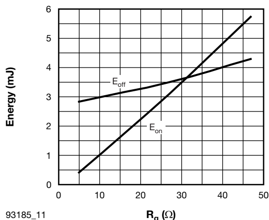
Fig. 11 - Typical IGBT Energy Loss vs. R_g T_J = 125^\circ\text{C} , I_C = 100\text{ A} , L = 500\text{ }\mu\text{H} , V_{CC} = 360\text{ V} , V_{GE} = 15\text{ V}
