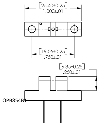
OPB854A3/OPB854B3 - Housing
