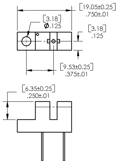
OPB854A2/OPB854B2 - Housing
