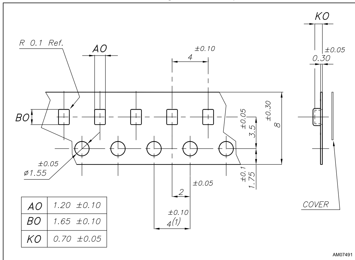
Figure 15. Carrier tape
