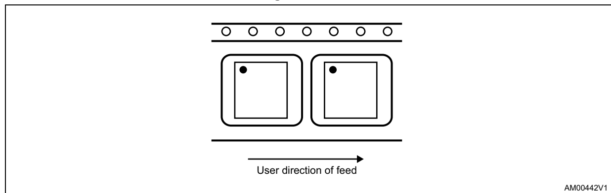
Figure 16. Pin 1 orientation
