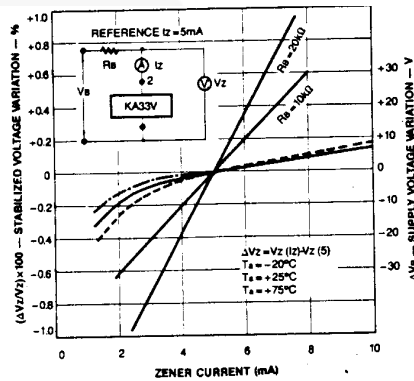
Figure 6. Stabilized Voltage Variation &amp; Supply Voltage Variation vs. Zener Current
