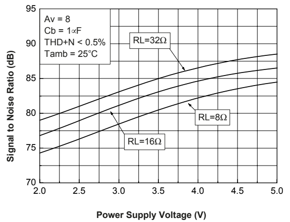
Figure 90. Signal to noise ratio vs. power supply voltage with weighted filter Type A
