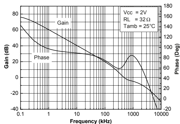
Figure 11. Open loop gain and phase vs. frequency RL = 32 \Omega , Vcc = 2 V
