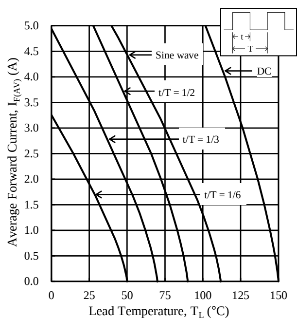
Figure 3. I_{F(AV)} vs. T_L ( T_J = 150 °C, V_R = 40 V)
