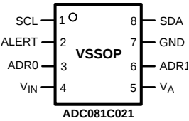
Figure 3. VSSOP – See Package Number DGK
