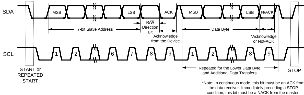
Figure 25. Basic Operation.
