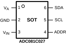
Figure 2. SOT (Addr Only) – See Package Number DDC
