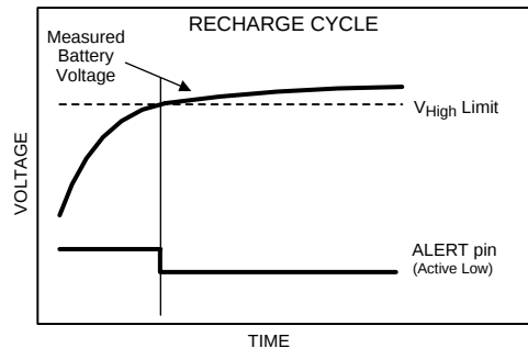
Figure 39. Recharge Cycle
