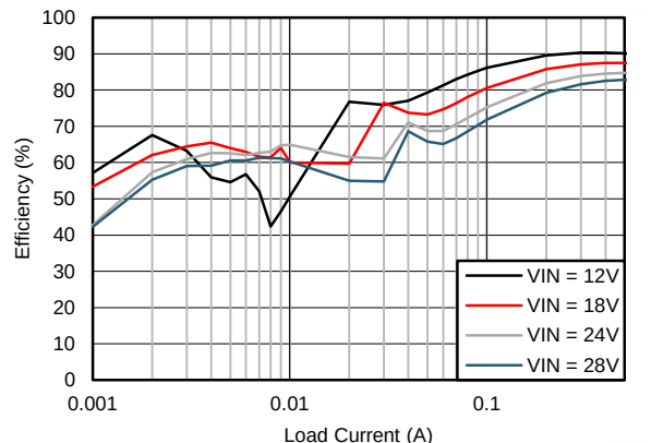
Figure 66. Efficiency
