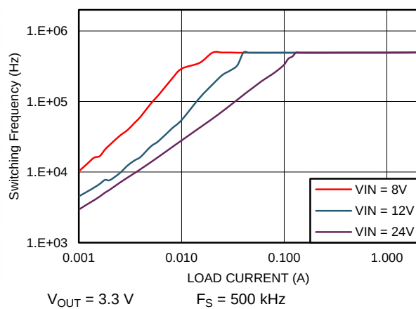
Figure 87. Switching Frequency vs I_{OUT} in PFM Operation
