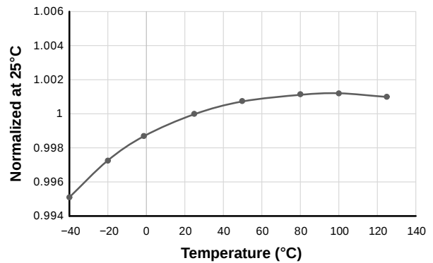
Figure 9. V_{\text{DD(OVP)}} vs. Temperature
