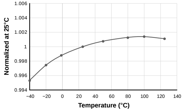
Figure 5. V_{\text{DIM(MAX)}} vs. Temperature
