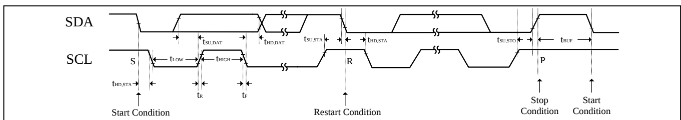
Figure 2 Interface timing
