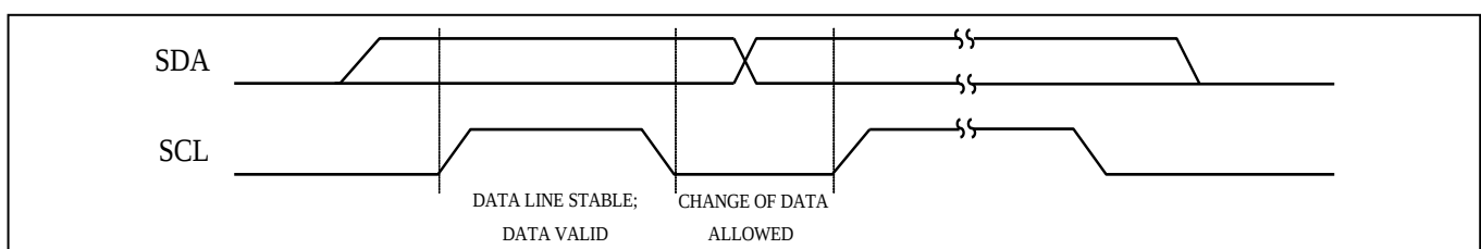
Figure 3 Bit transfer
