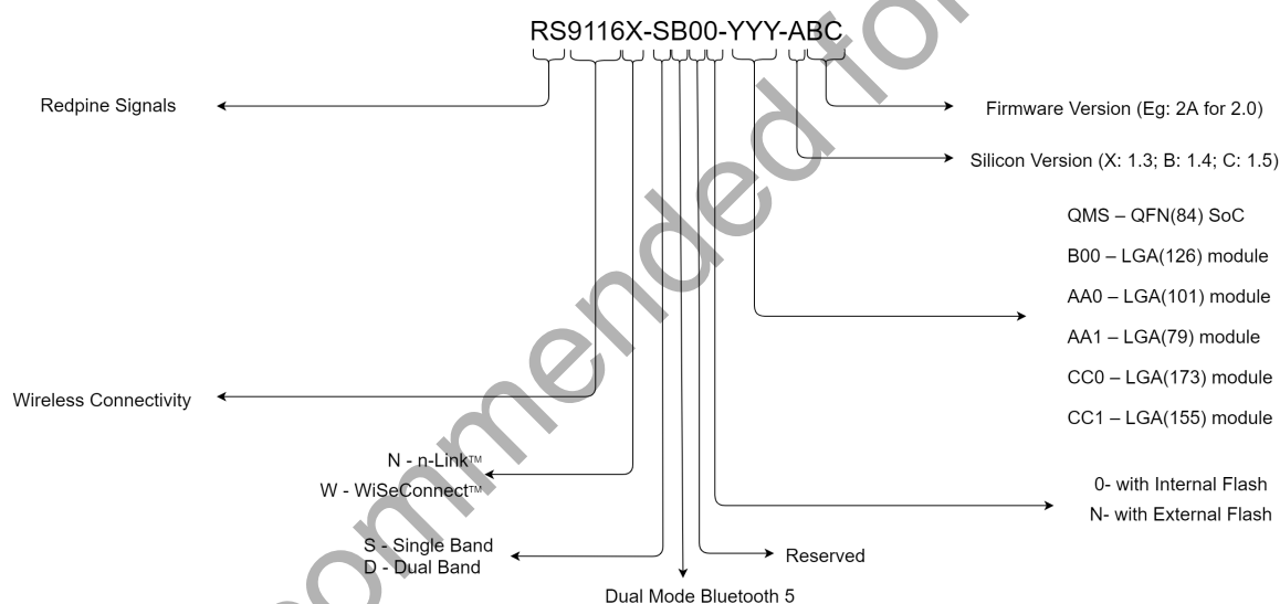
Figure 34 Device Nomenclature
