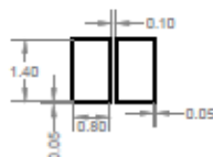
Soldermask opening details
