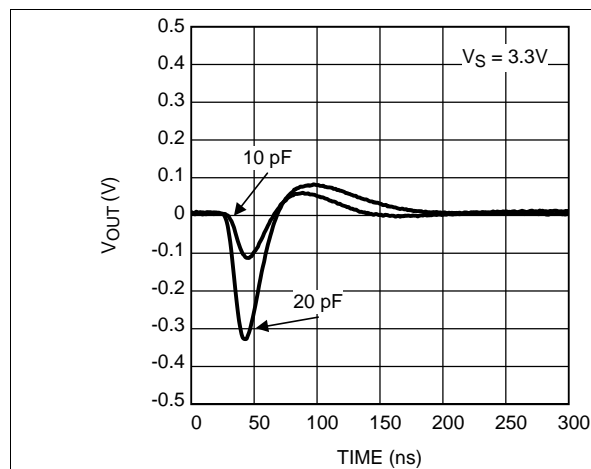
Figure 57. Capacitive Load Response at 3.3 V
