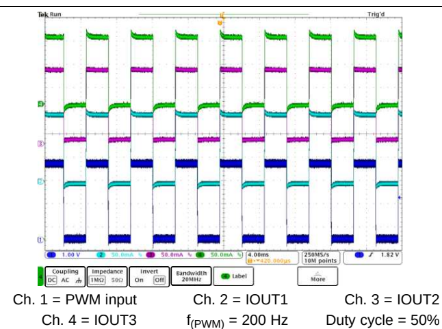
Figure 10. PWM Dimming
