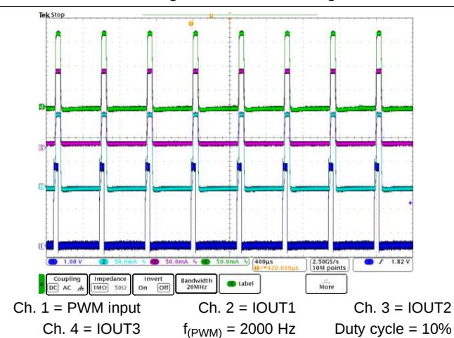
Figure 12. PWM Dimming
