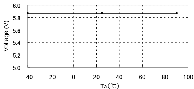
ZCD Voltage Clamp vs. Temperature Upper side
