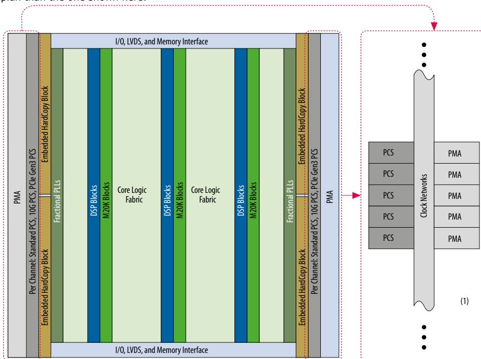
Figure 1. Stratix V GT, GX, and GS Device Chip View
