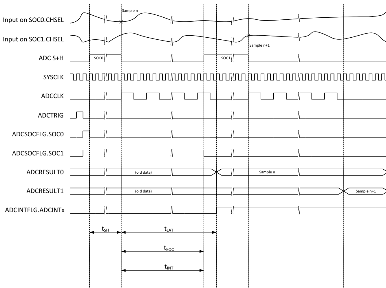
Figure 7-39. ADC Timings for 12-Bit Mode
