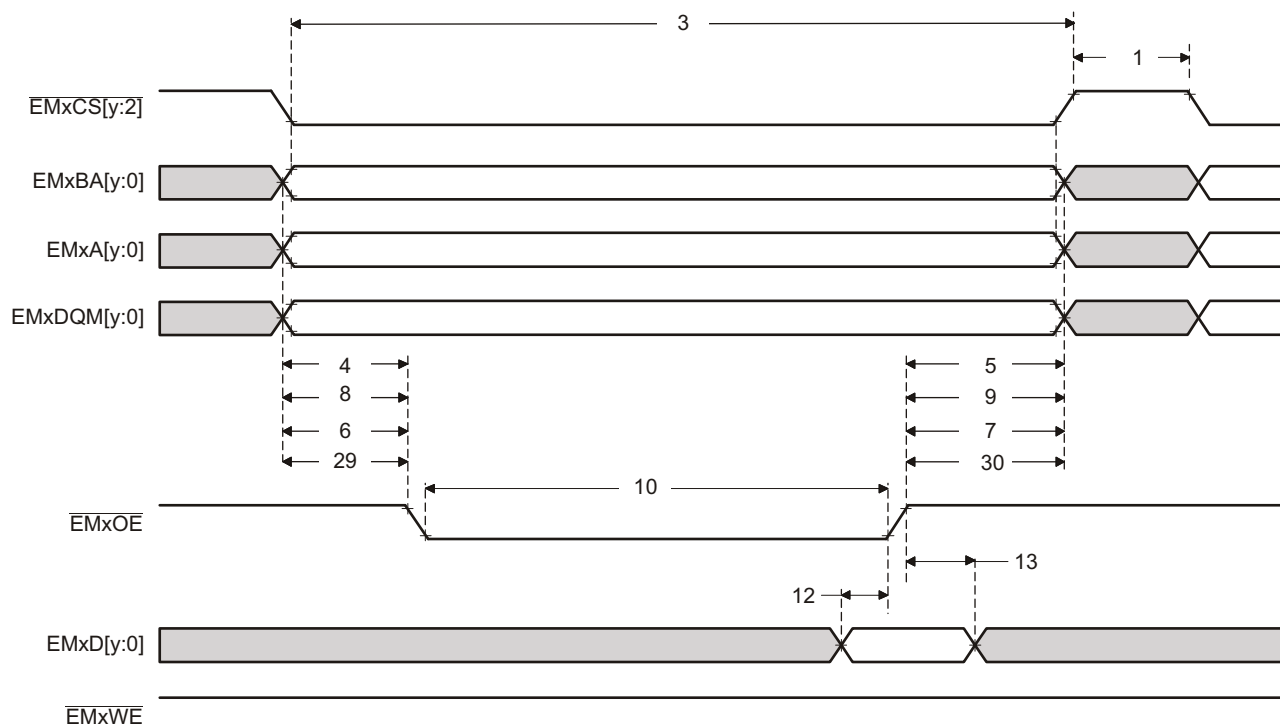
Figure 7-26. Asynchronous Memory Read Timing
