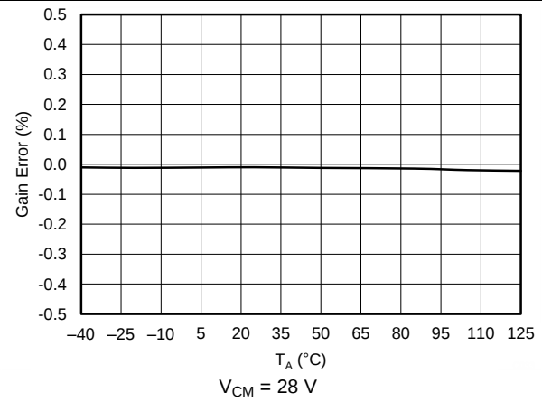
Figure 38. Current Sense Gain Error vs Temperature
