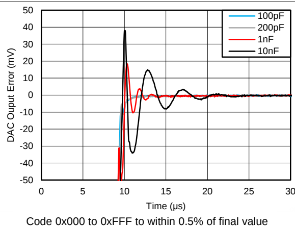
Figure 108. DAC Settling Time
