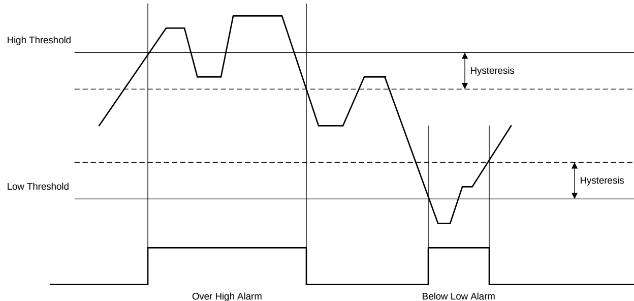
Figure 59. Device Hysteresis
