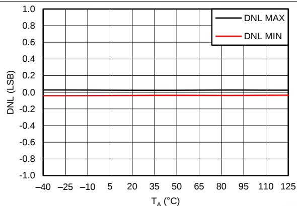
Figure 12. Bipolar DAC DNL vs Temperature
