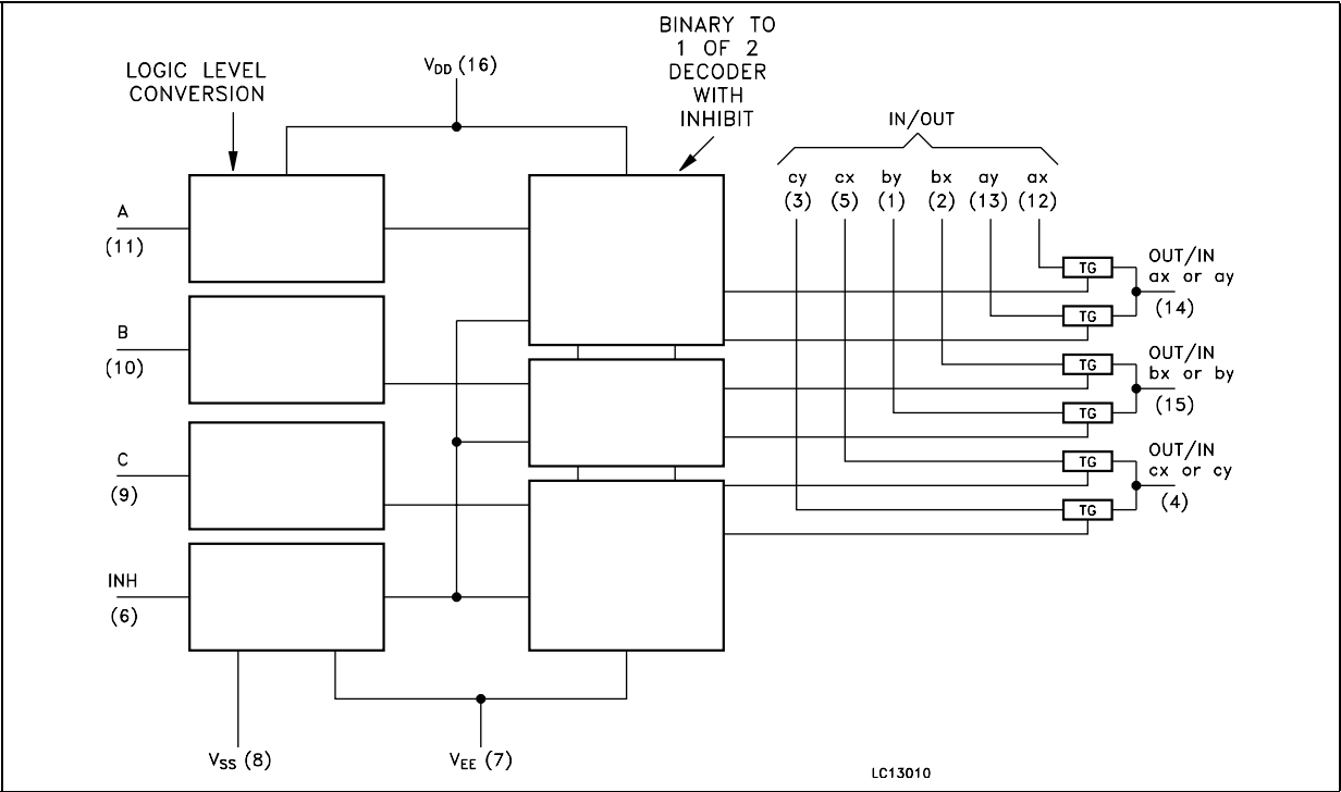
Figure 3: Functional Diagram
