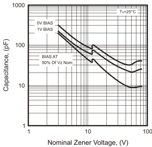
Fig.4 - Typical Capacitance
