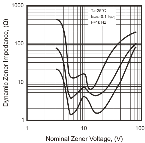
Fig.2 - Effect Of Zener Voltage On Zener Impedance
